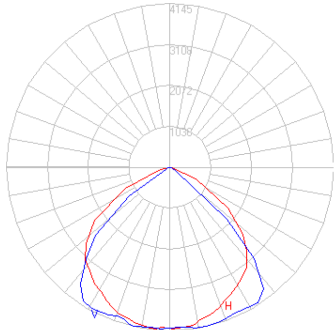
EHF-FLOOD-5050K-277
