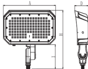
(Knuckle)
