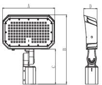
(Slip-fitter)
